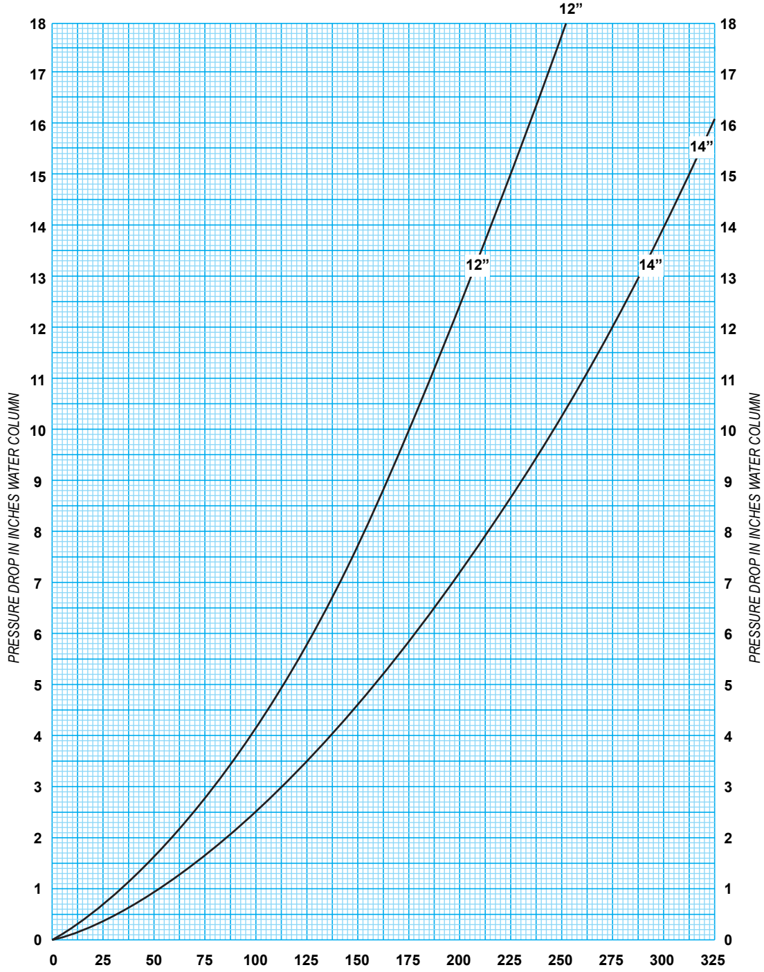
FLOW CURVE FOR PRISM SSDFA MODELS: 12"/14" OSDF/OSSF
